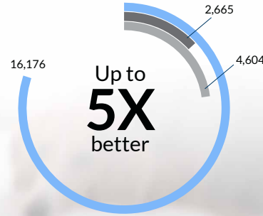
Futuremark® 3DMark®
